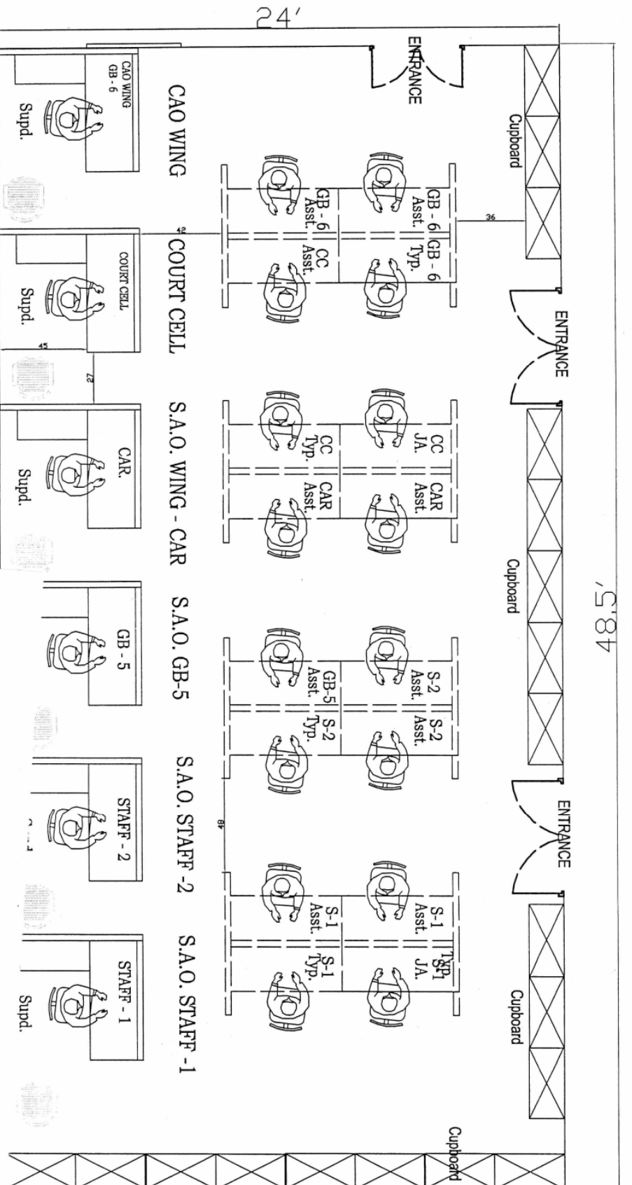
PROPOSED DRAWING FOR - DIG - OFFICE CAO WING GB - 6, COURT CELL, S.A.O WING - CAR, GB - 5, STAFF
